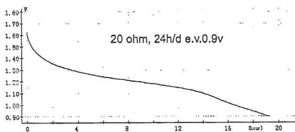
Chart 1. Discharge diagram
